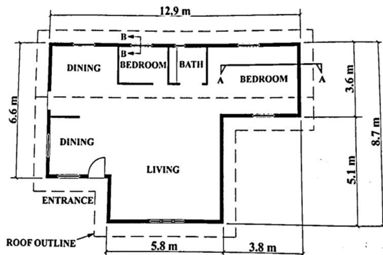
Figure 1. Floor plan
